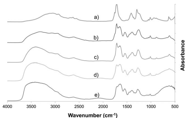
Figure 5. FTIR spectra of gelatin solutions (400 mg/mL) at different acetic acid concentrations (% v/v): (a) glacial acetic acid; (b) 100%; (c) 75%; (d) 50%; and (e) 25%.
