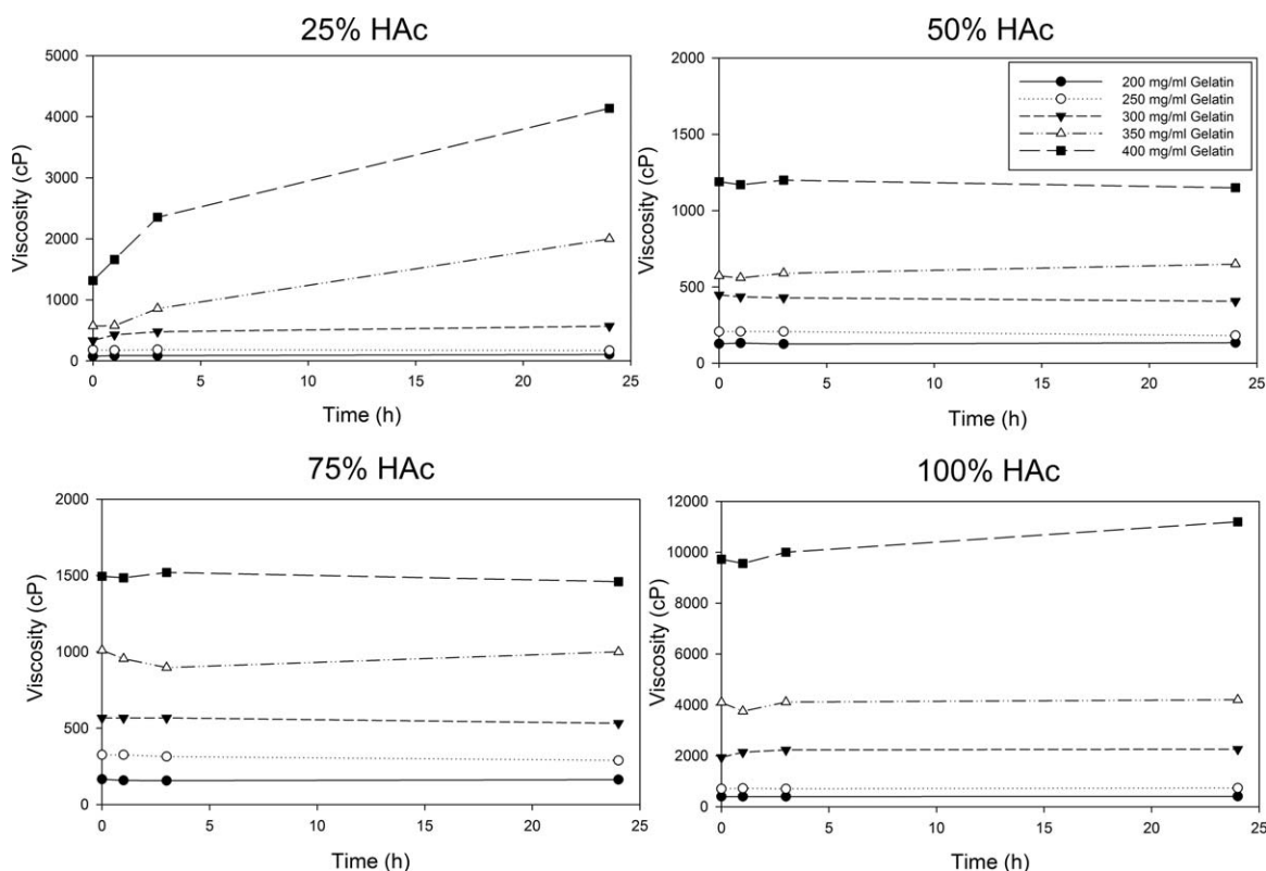
Figure 1. Viscosity changes with storage time for solutions of different gelatin and acetic acid concentrations. All viscosity values have a standard deviation below 2%.
