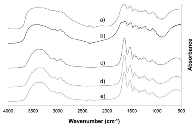
Figure 6. FTIR spectra of electrospun gelatin fibers obtained from solutions containing 300 mg/mL of gelatin and different acetic acid concentrations (% v/v): (a) powder gelatin; (b) 100%; (c) 75%; (d) 50%; and (e) 25%.
