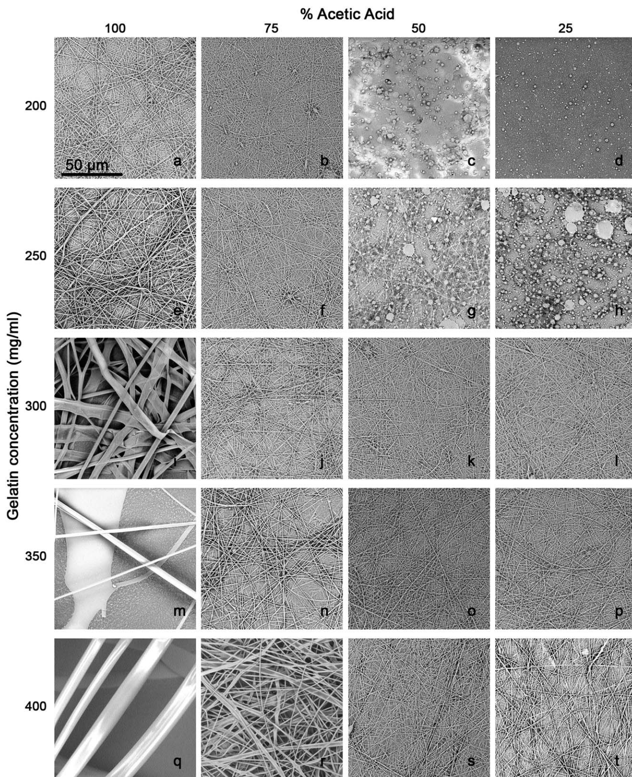
Figure 2. SEM images of electrospun gelatin fibers as a function of Acetic Acid percentage (100, 75, 50 and 25, arranged in columns) and Gelatin concentration in mg/ml (200, 250, 300, 350 and 400, arranged in rows). For instance, image (f) corresponds to fibers fabricated with 75% Acetic Acid and 250 mg/ml of Gelatin. The scale bar shown in microphotography (a) is valid for all the images.
