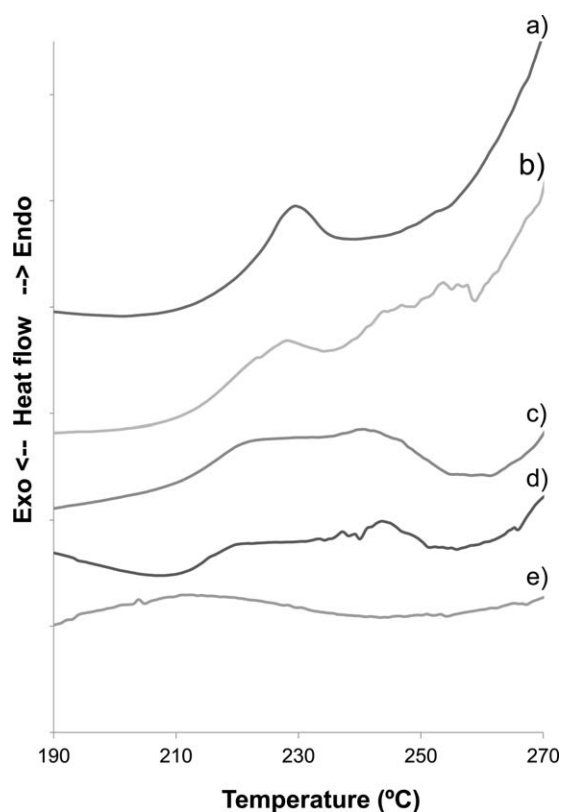
Figure 7. DSC of electrospun fibers obtained for solutions containing 300 mg/mL gelatin and different acetic acid concentrations (% v/v): (a) powder gelatin; (b) 25%; (c) 50%; (d) 75%; and (e) 100%.
